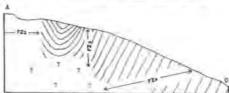
FIG. 5 GEOLOGICAL PROFILES FOR THE GUNBERT ROAD SITE
