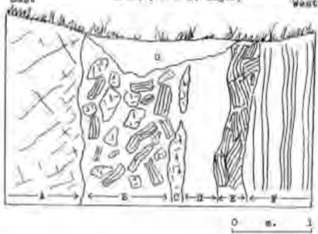
FIG. 5 SKETCH OF DOLERITE-STRETTON SHALE FAULT
