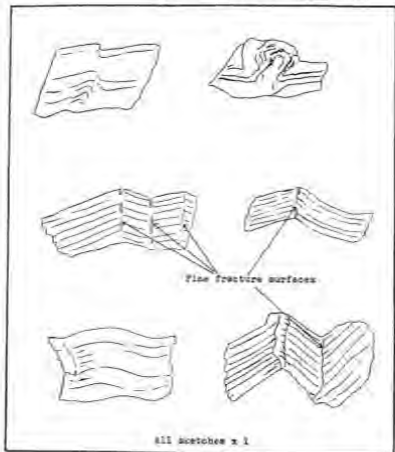
FIG. 4 SKETCHES OF FOLD STRUCTURES AND LINE-BANDS DEVELOPED AT THE CUNNEY ROAD SITE
