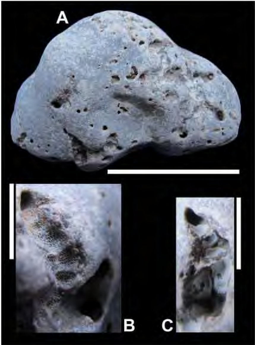
Figure 6: RGM.1332371, corraded limestone clast with remnants of a mature Entobia isp. that has provided protected environments for encrusting invertebrates. (A) Surface of clast. Scale bar represents 50 mm. (B) Bryozoan colony encrusting 'scalloped' chambers of Entobia . (C) Basis plates of Balanus sp. encrusting 'scalloped' chambers of Entobia . Specimen uncoated. Scale bars represent 10 mm unless stated otherwise.
