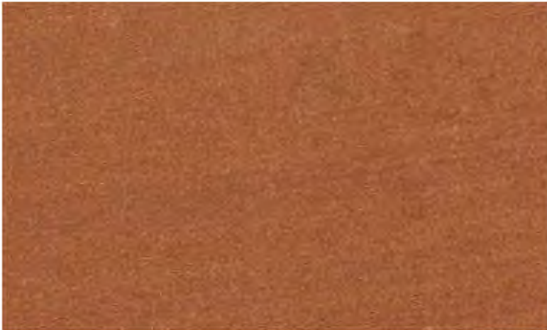
Figure 10: St Bees Sandstone
