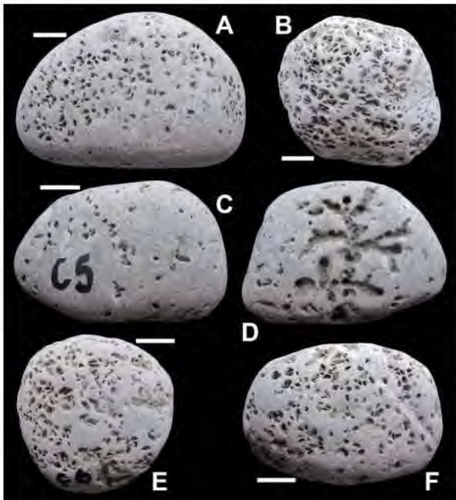
Figure 2: Mainly Caulostrepsis isp. cf. C. taeniola Clarke, 1908.
