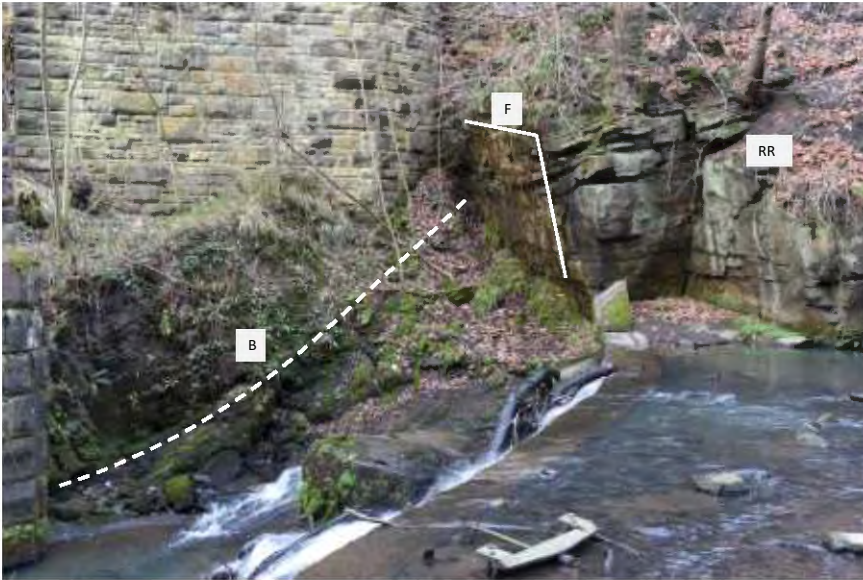
Figure 14: Fault near the abutment of the railway bridge. RR = Rough Rock; F = location of fault plane; B = line following planes of bedding in the shales.
