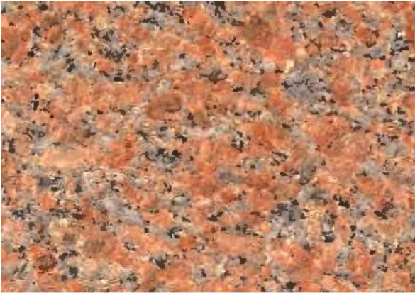
Figure 7: Corrennie pink granite
