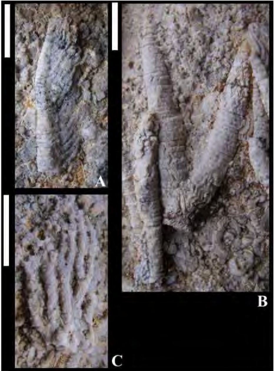
Figure 3: BMNH EE16661. (A, B) Woodocrinus macrodactylus de Koninck, 1854.
