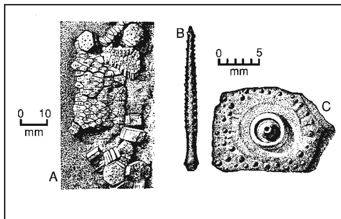
Figure 9. Echinoids of the Clitheroe area.
