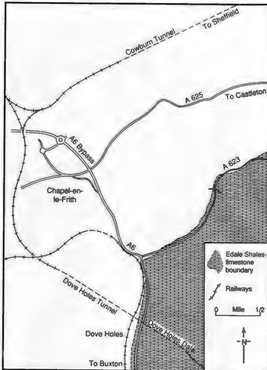
Figure 6. The Dinantian-Namurian boundary in the vicinity of the Dove Holes tunnel
